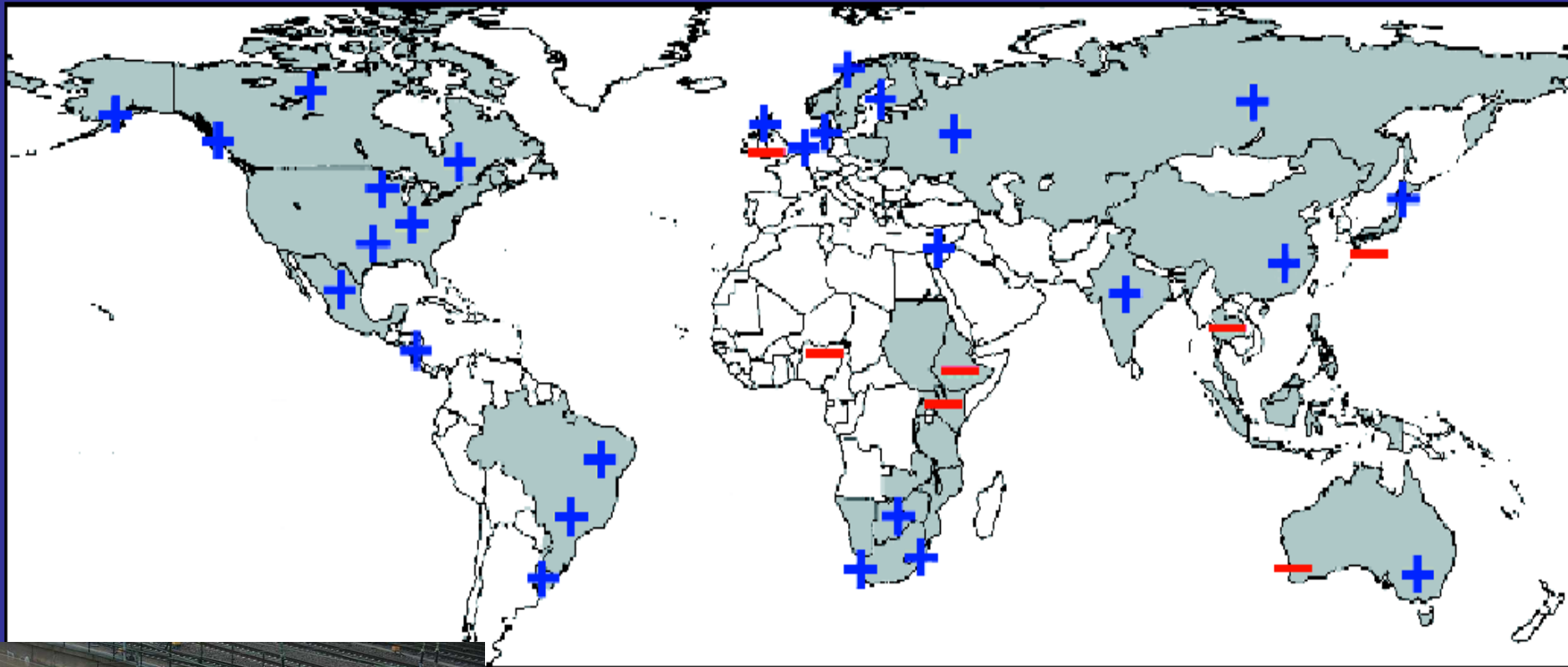
Regions of disproportionate changes in heavy (95 th ) and very heavy (99 th ) precipitation
